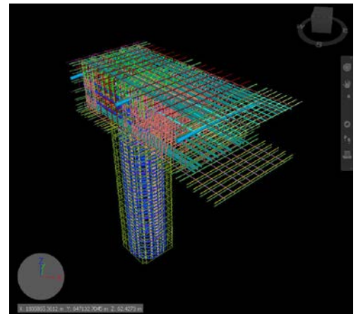
Yerba Buena Island Ramps – San Francisco, CA Client: Golden State Bridge – Created and coordinated integrated rebar shop drawings using 3D models made in Revit and Microstation for the new Bay Bridge Yerba Buena Island off-ramps.
